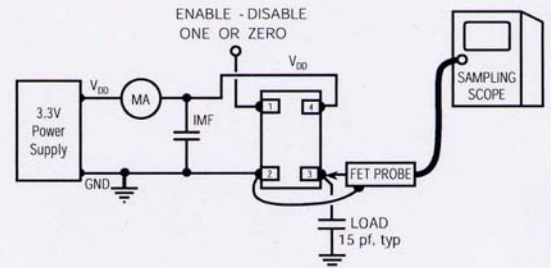
Fig. 4. Test Circuit
